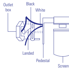
ELECTRIC DIAGRAM (W) White wire: Neutral (B) Black wire: Line (⊕) Copper wire: Ground
